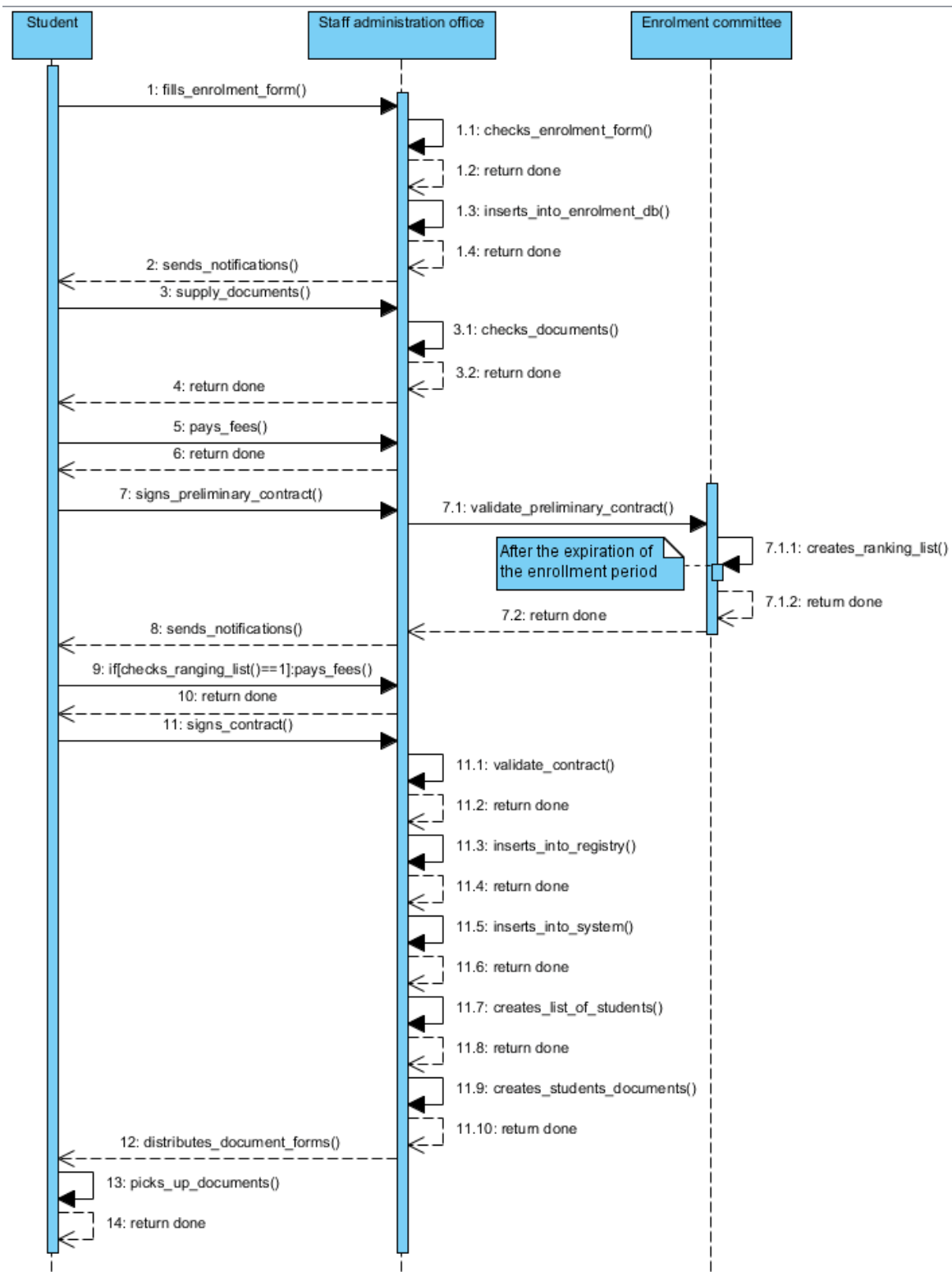
Figure 7. Sequence Diagram.
