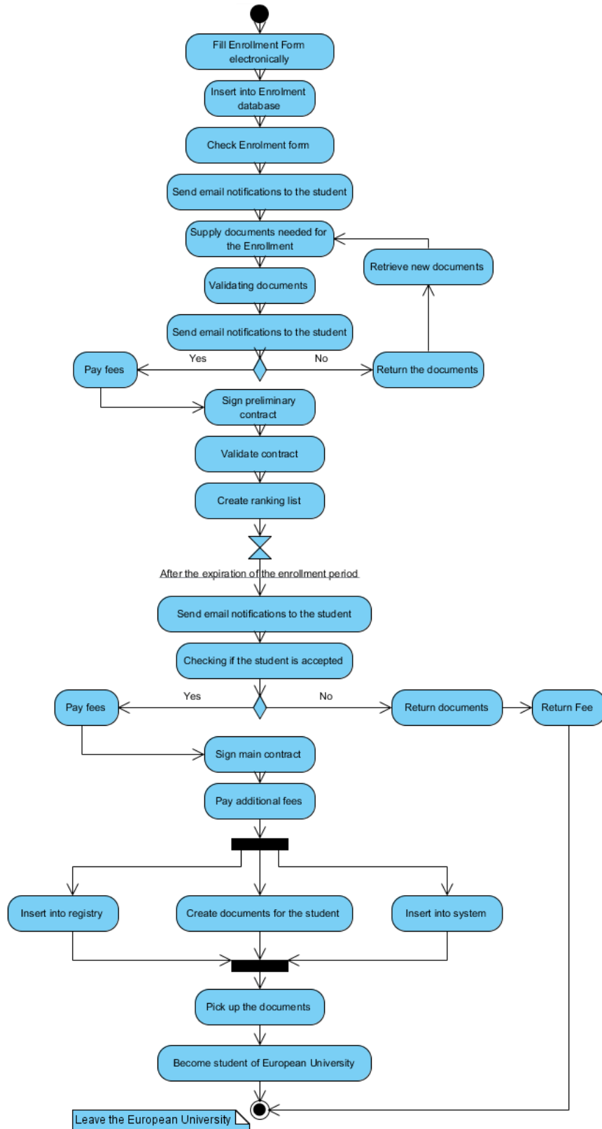
Figure 5. Activity diagram.
