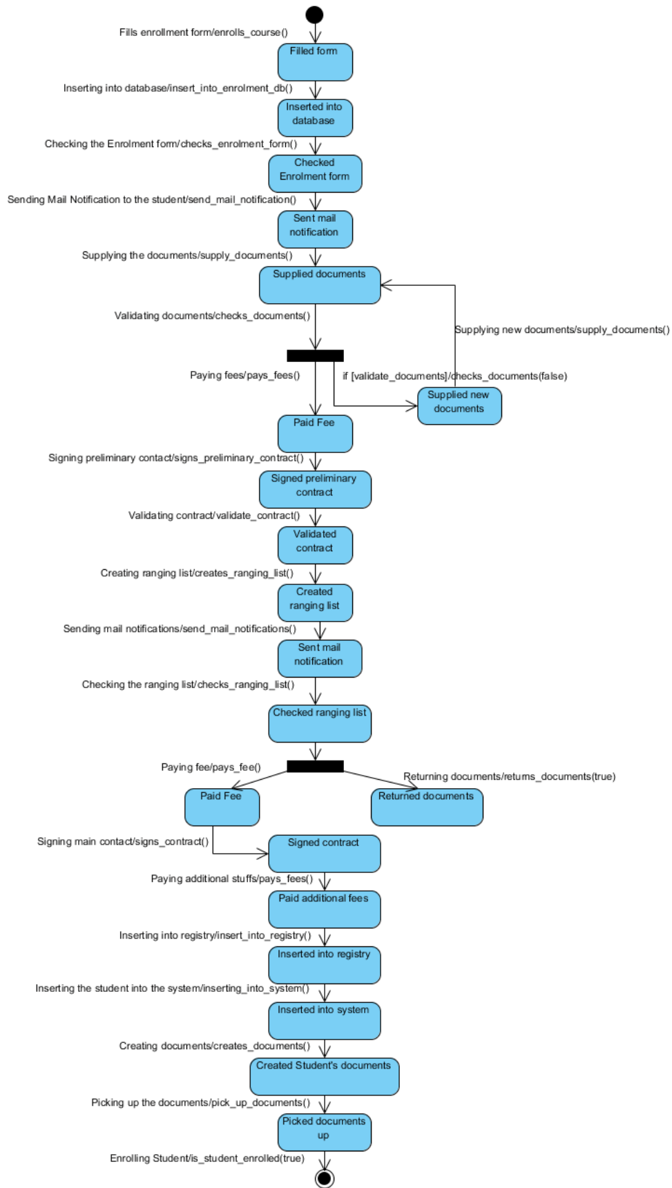
Figure 6. State Machine Diagram for the Enrolment Application entity.
