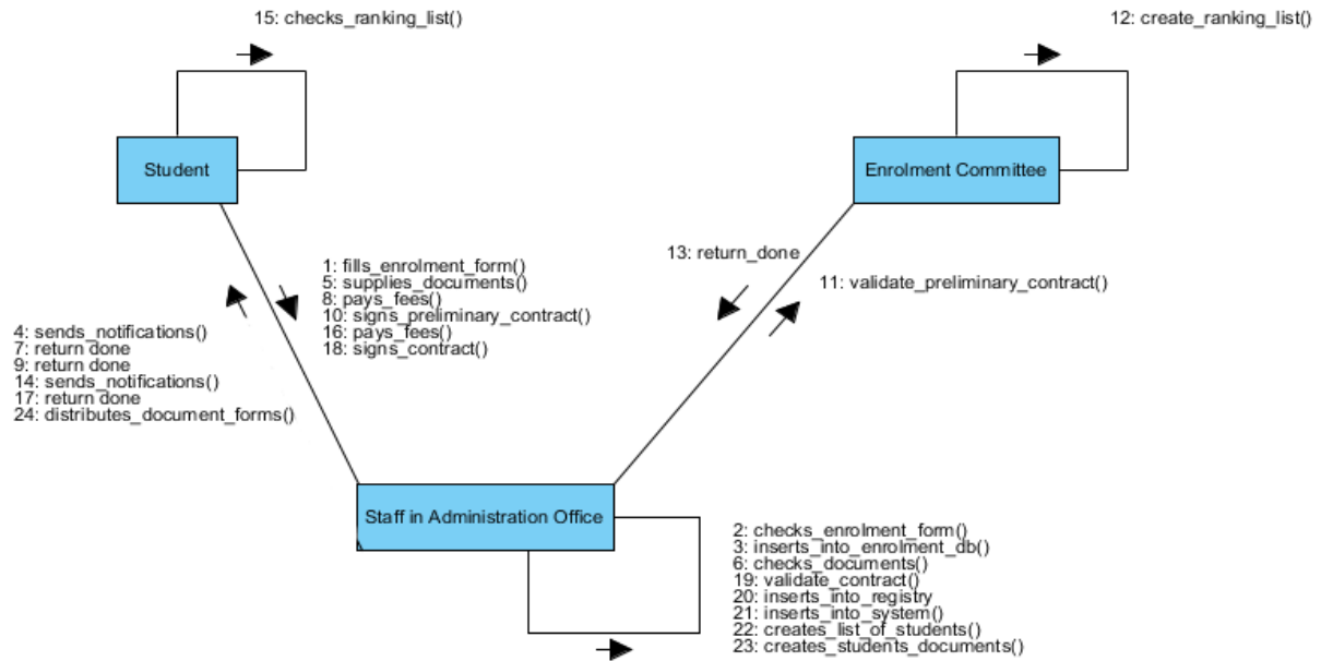
Figure 8. Collaboration Diagram.
