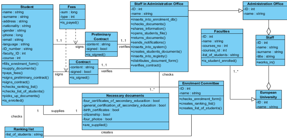
Figure 9. Class diagram.
