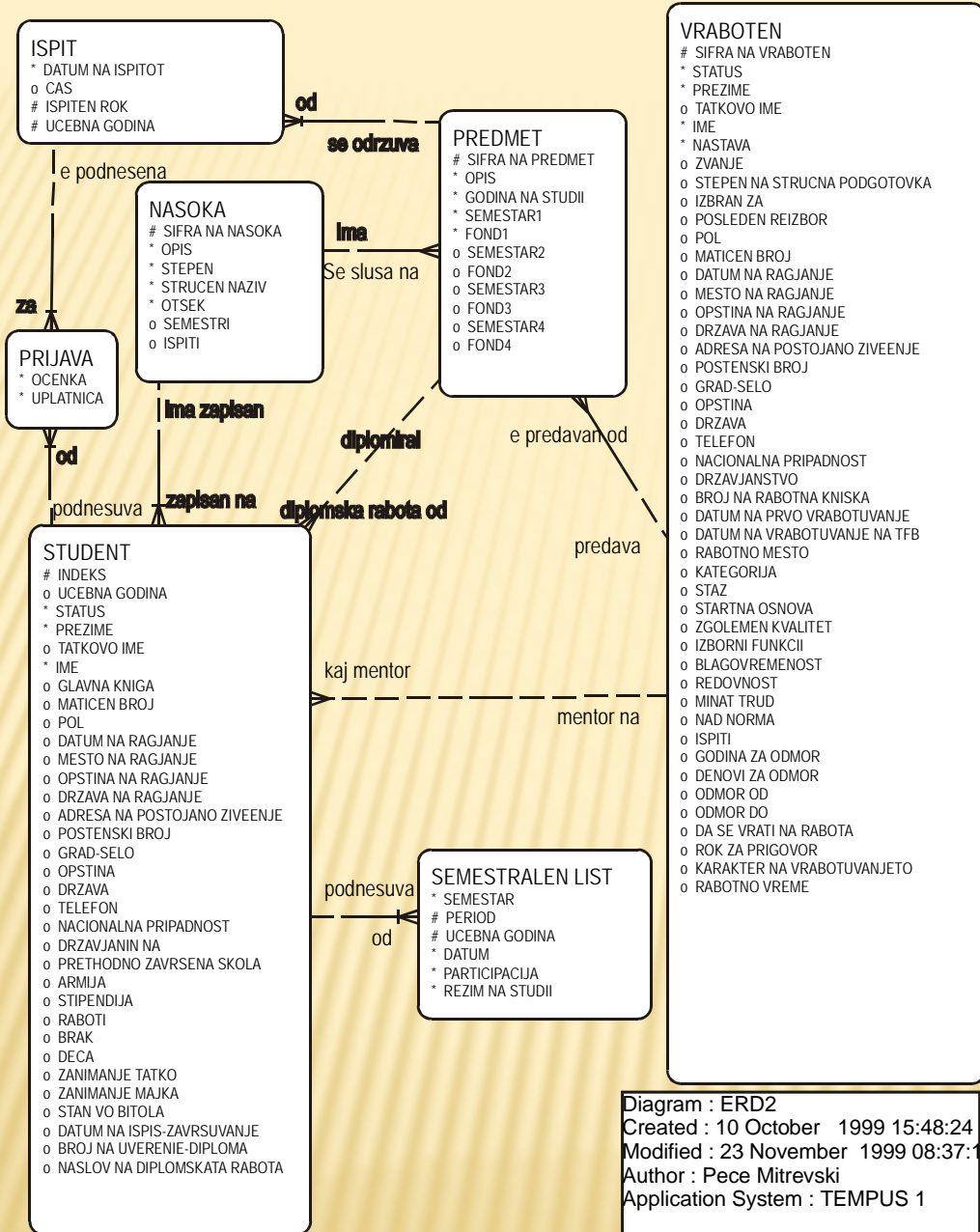
Entity – relationship diagram
